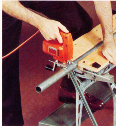
Horizontal V-grooves grip tubular objects.
