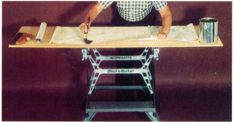
2' x 6' x 1/2" piece of plywood mounted on a 2x4 three feet long, placed in vise jaws, makes a table for paper hanging jobs.
