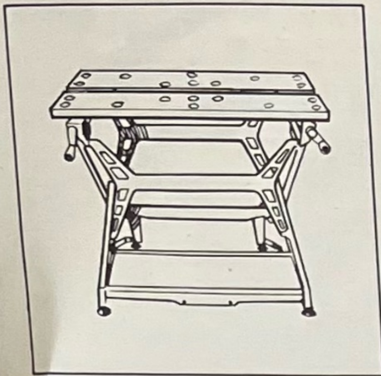
Single height (model WM225) has a working height of 23 1/4" (590mm)—the comfortable height for the vast majority of jobs.
