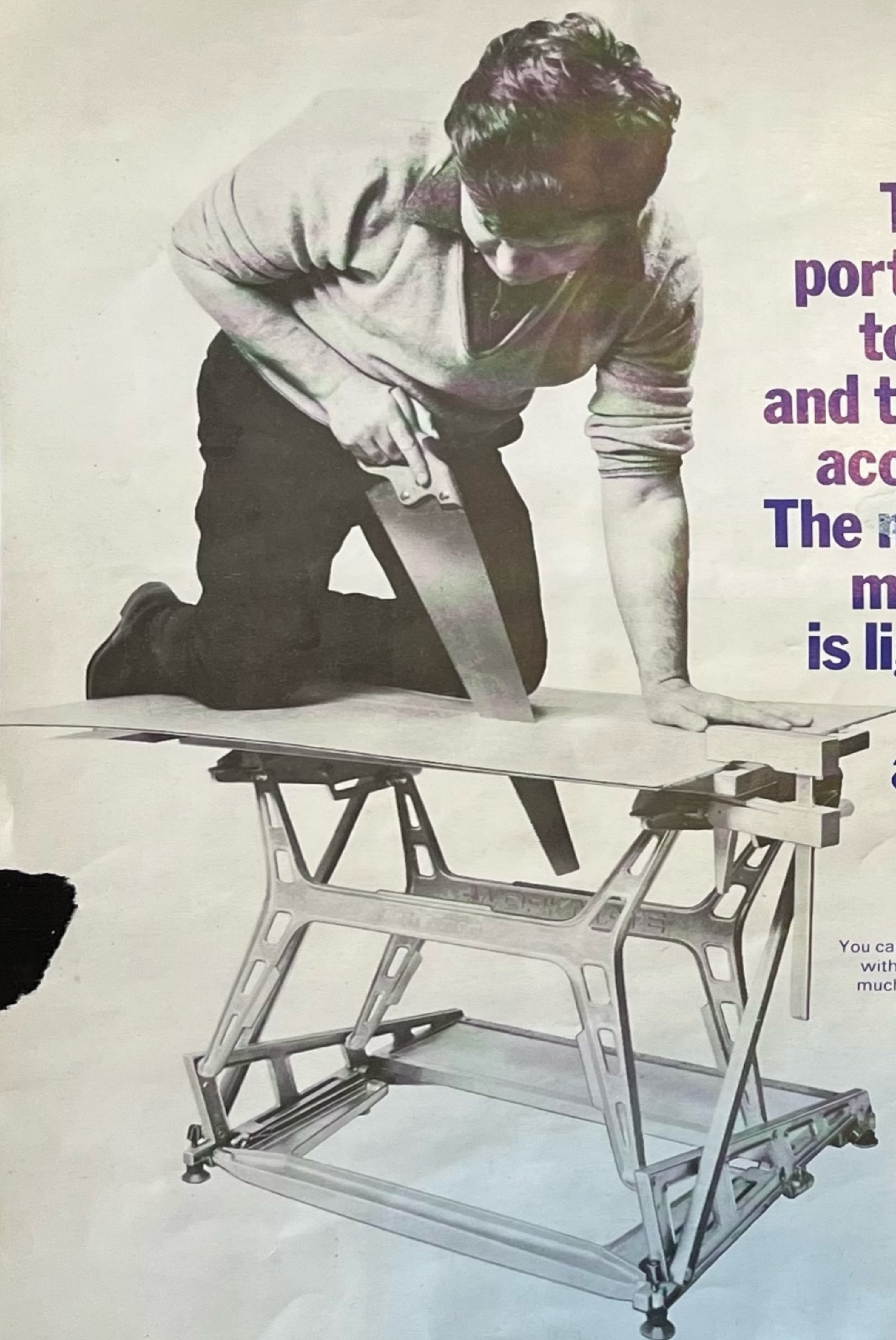
Dual height professional (model WM325) has folding lower legs for added versatility offering two working heights of 23 1/4" (590mm) and 32 1/4" (820mm). A kit of legs to convert the WM225 to a dual height WM325 is available, catalogue number WM275.
