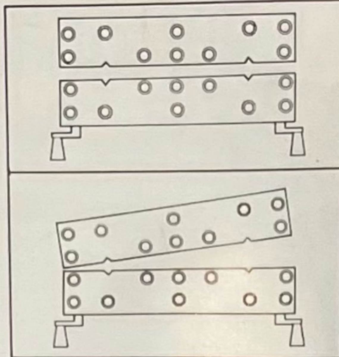
The giant 29" (740mm) vice has a control screw at each end, enabling parallel or tapered material to be held securely.
