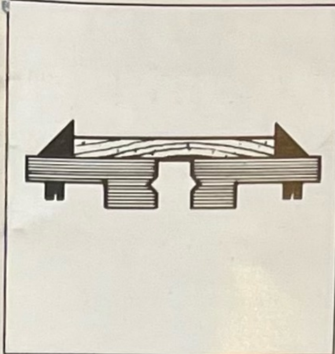
Four vice pegs are provided free with the Workmate. These fit into a series of holes in the vice bars, and effectively more than double the normal 4" (100mm) vice capacity. They are ideal for holding irregularly shaped work pieces.
